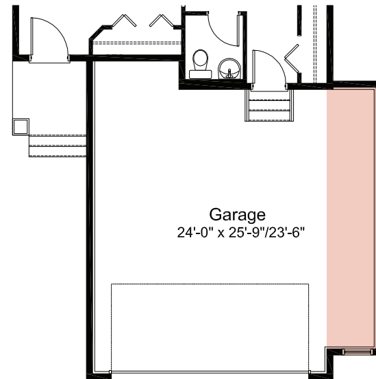
4' Garage Width Extension Option
