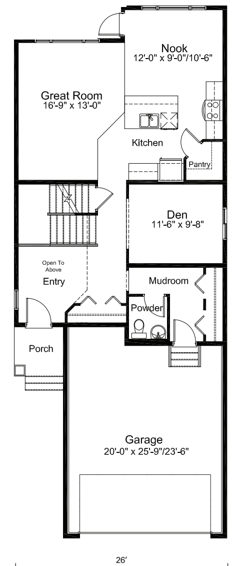
Main Floor 996 sq. ft.
