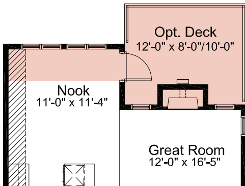
Fireplace Option with 2' Nook Extension (Adds 24 Sq.Ft. to Main and Foundation)
