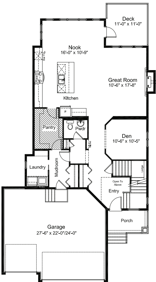
Main Floor 1321 sq. ft.
