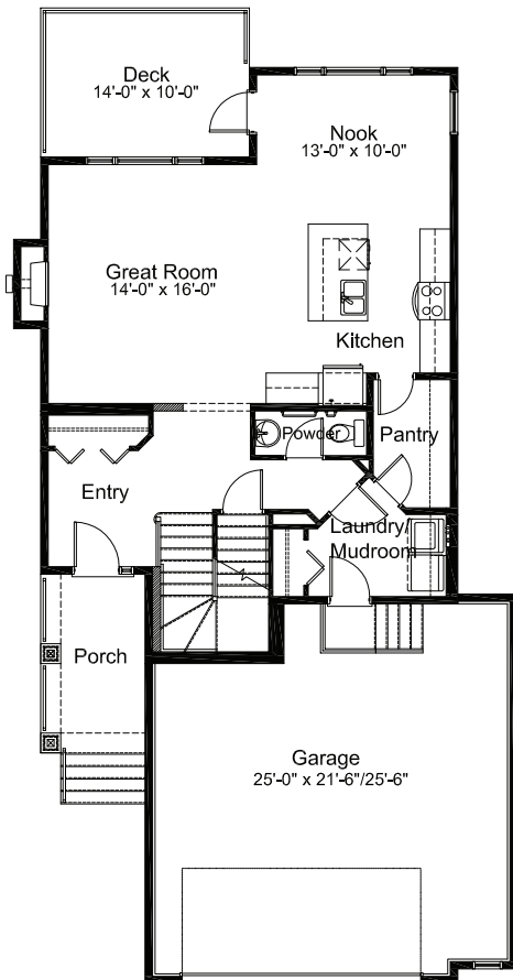
Main Floor 947 sq. ft.
