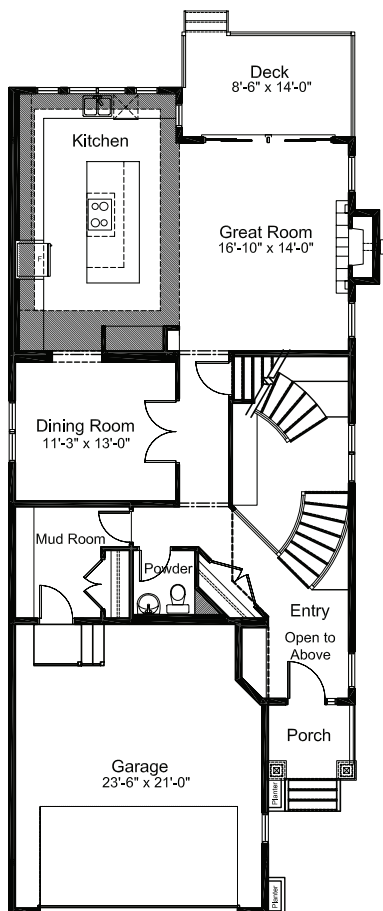
Main Floor 1,223 sq. ft.
