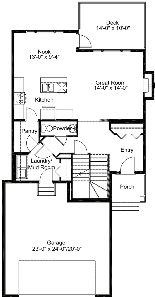
Main Floor 863 sq. ft.
