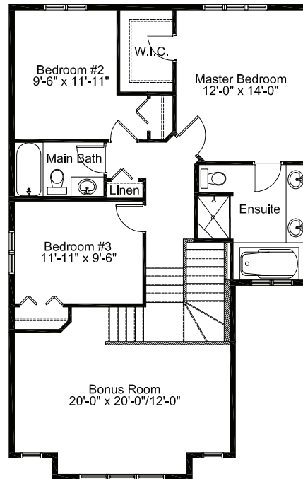
Upper Floor 1089 sq. ft.
