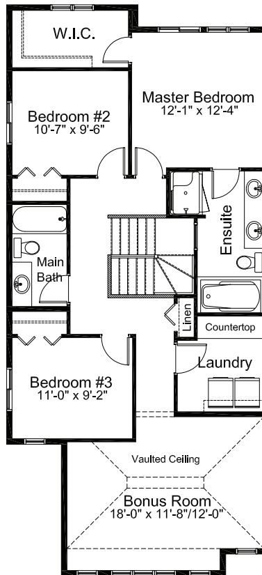
Upper Floor 1156 sq. ft.
